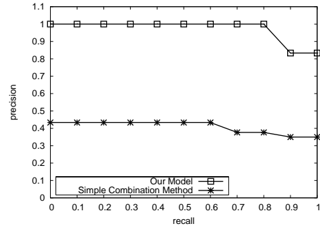
Figure 5: Precision/Recall for information need 2
