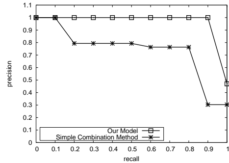
Figure 4: Precision/Recall for information need 1
